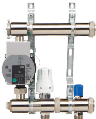
Compact Mixing Circuit
