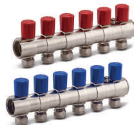
Brass 1" Completed Type Manifold - (Eco)
