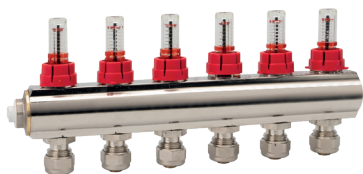
Brass 1" Flow Meter Manifold (16X2)
