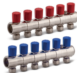
Brass 1" Completed Type Manifold - (Eco)
