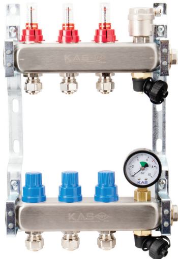
1" Stainless Steel Manifold With Automatic Air Vent
